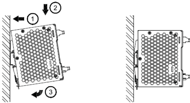
Fig. 3.1 Mounting
