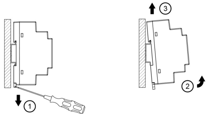
Fig. 2.2 Dismounting
