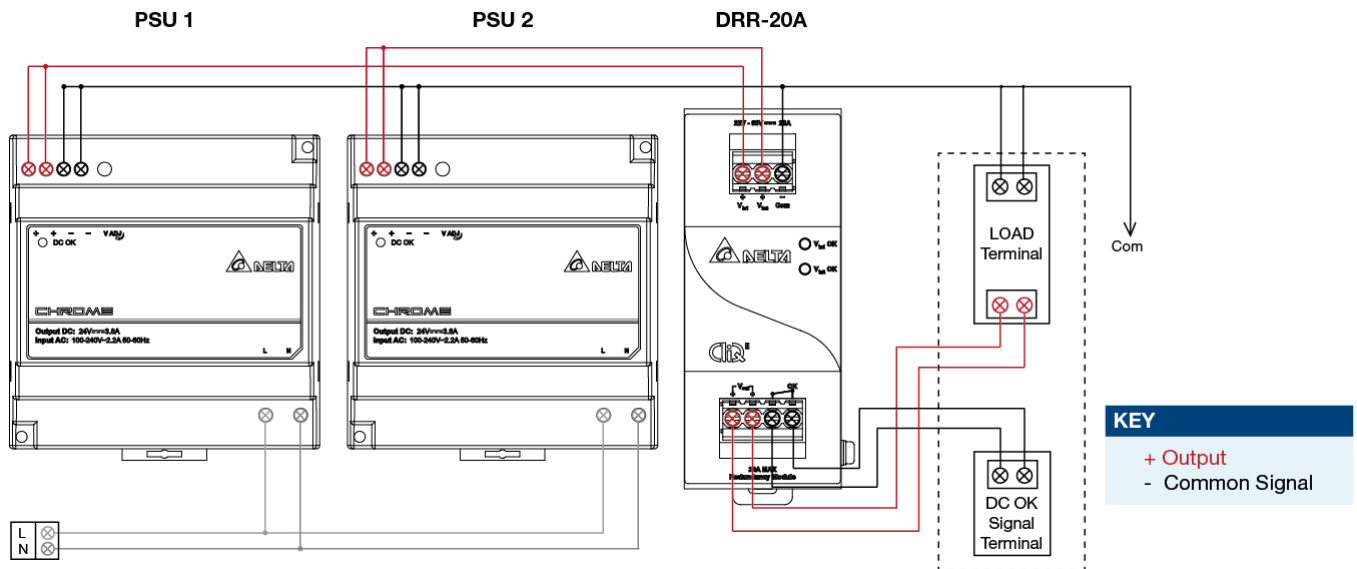
Fig. 3 Redundancy / Parallel Operation Connection Diagram
