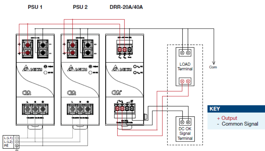
Fig. 2.1 Redundancy / Parallel Operation Connection Diagram
