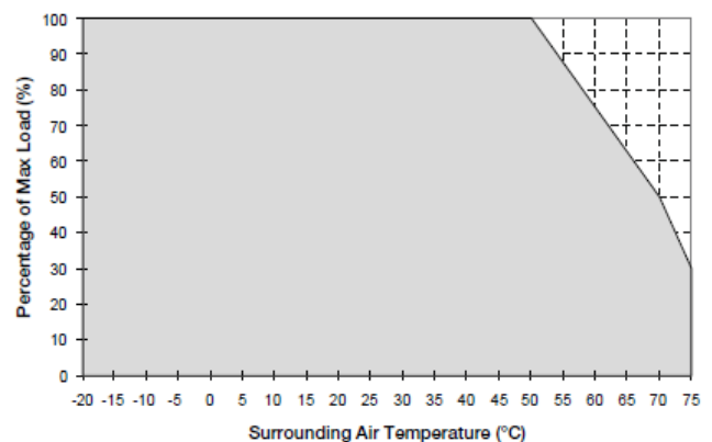
Fig. 1.2 De-rating for Horizontal Mounting Orientation > 50°C de-rate power by 2.5% / °C, > 70°C de-rate power by 4% / °C
