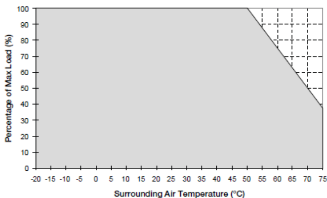
Fig. 1.1 De-rating for Vertical Mounting Orientation > 50°C de-rate power by 2.5% / °C
