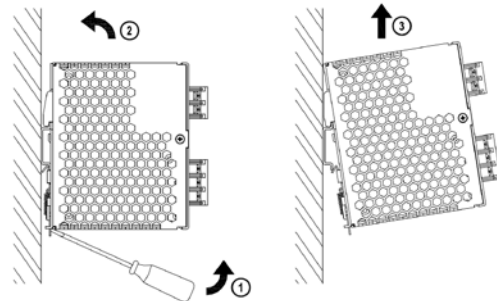
Fig. 2.2 Dismounting
