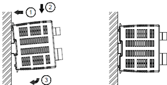
Fig. 2.1 Mounting
