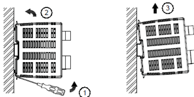
Fig. 2.2 Dismounting
