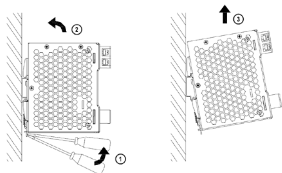
Fig. 2.2 Dismounting
