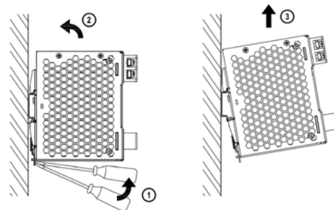
Fig. 2.2 Dismounting
