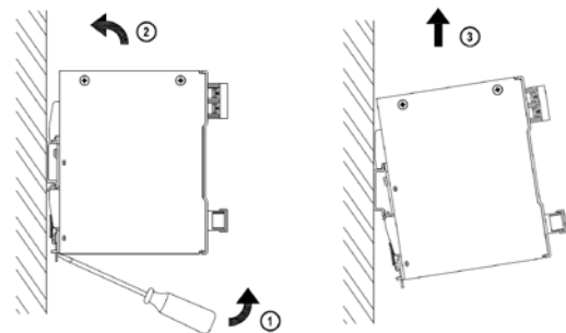
Fig. 2.2 Dismounting
