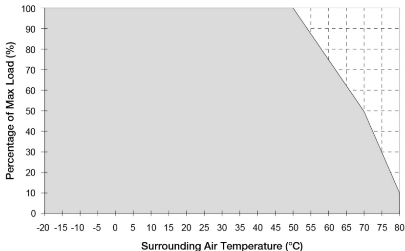
Fig. 1 De-rating for Vertical Mounting Orientation > 50°C de-rate power by 2.5% / °C, > 70°C de-rate power by 4% / °C
