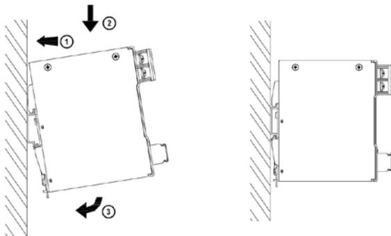
Fig. 2.1 Mounting
