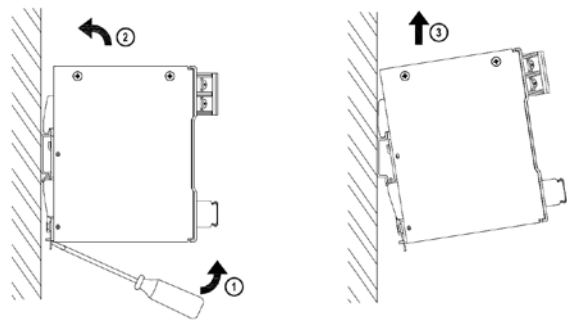
Fig. 2.2 Dismounting
