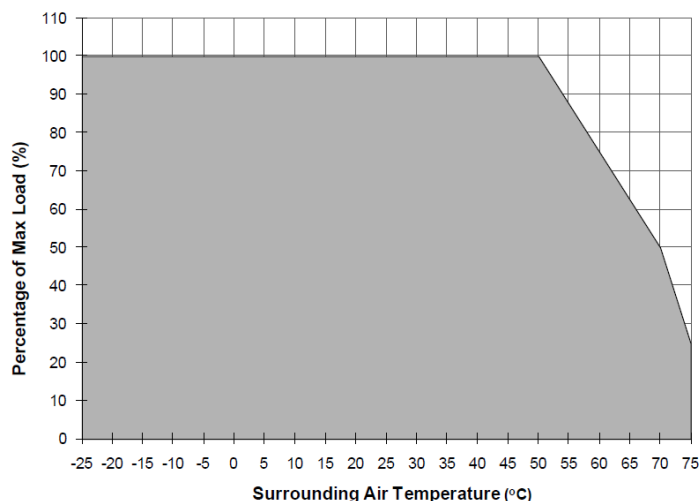
Fig. 1.1 De-rating for Vertical Mounting Orientation > 50°C de-rate power by 2.5% / °C > 70°C to 75°C de-rate power by 5% / °C
