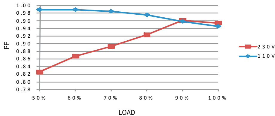
Constant Current Mode
