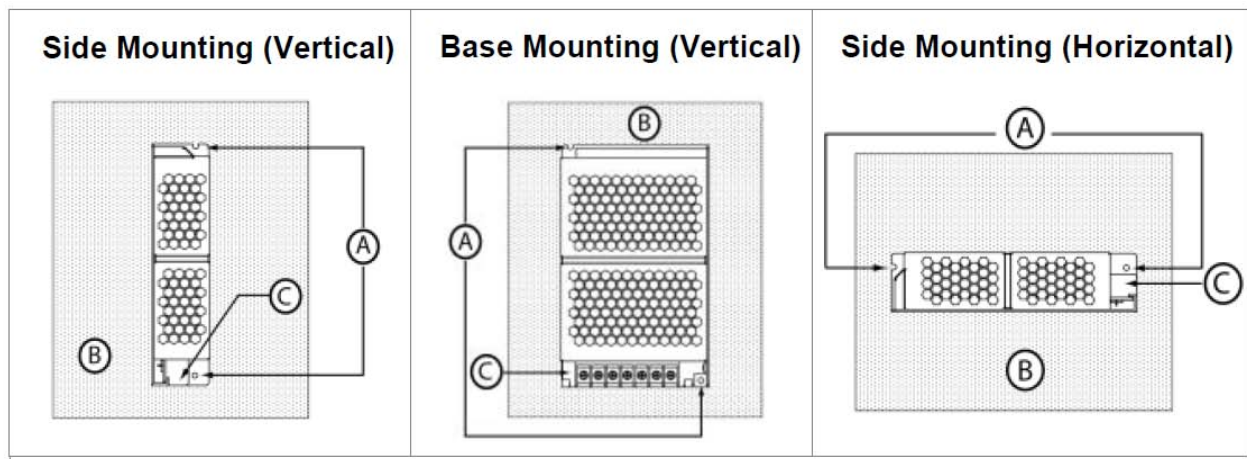
Fig. 2 Mounting Orientation
