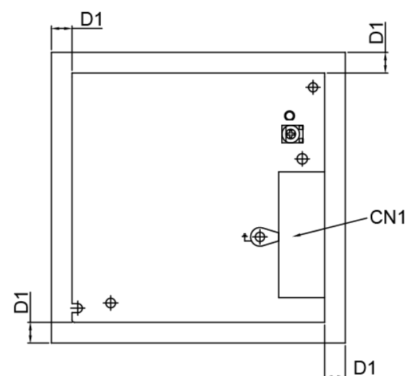
Fig. 3 Assembly Reference
