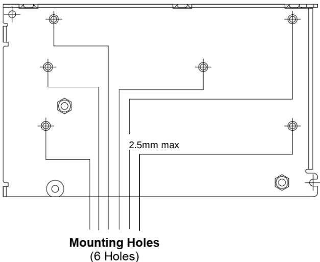
Fig. 3 Mounting Hole Locations
