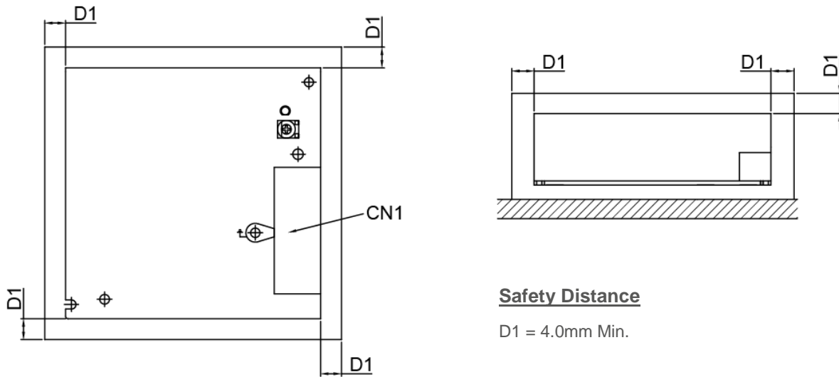
Fig. 3 Assembly Reference
