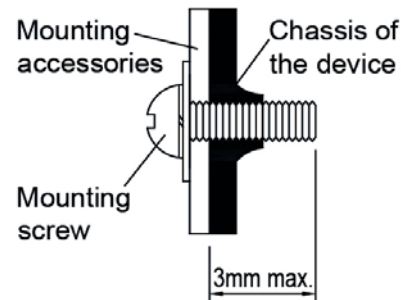
Fig. 4 Mounting Screw
