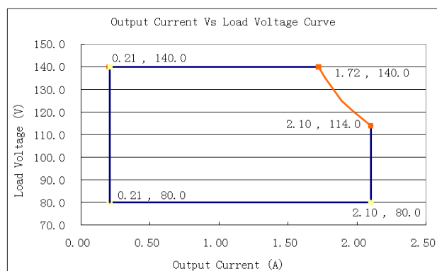
LDP-240X368-B
