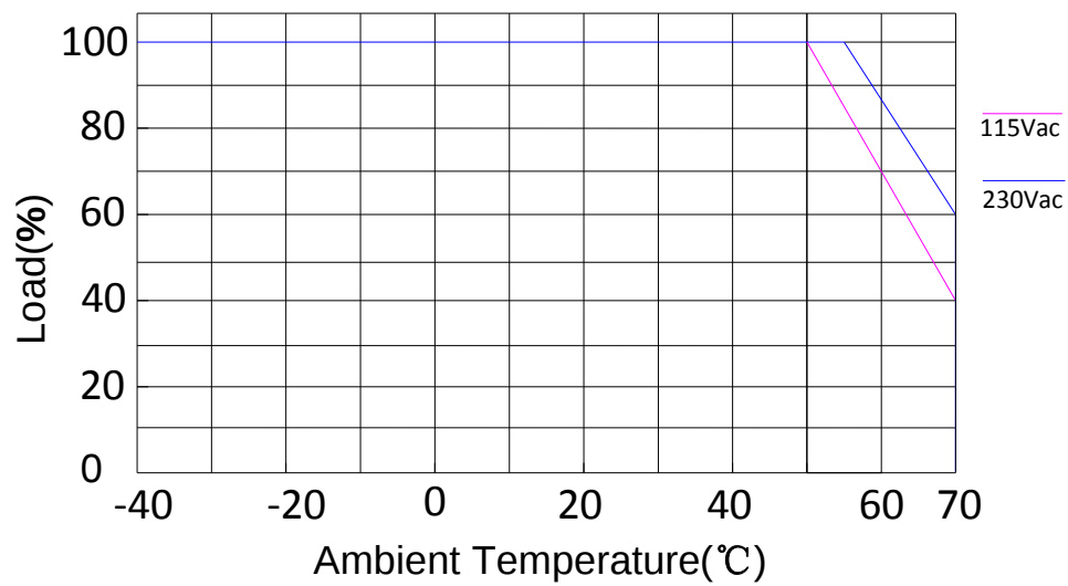
Derating Curve
