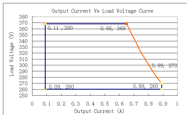
LDP-240X368-B
